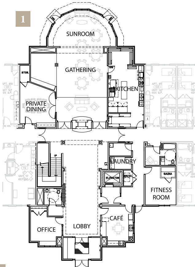
1 Main Level
